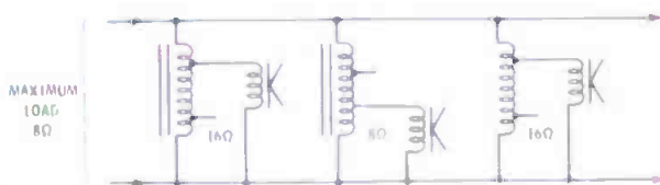
Fig. 3 Gates' suggestions on using their speaker matching transformer.
