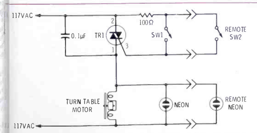
Fig. 4 Turntable switch used at WHCN-FM. The triac is a IRT82-C.
