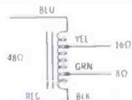
UP TO 6 MAY BE PARALLELED TO OBTAIN 8Ω
