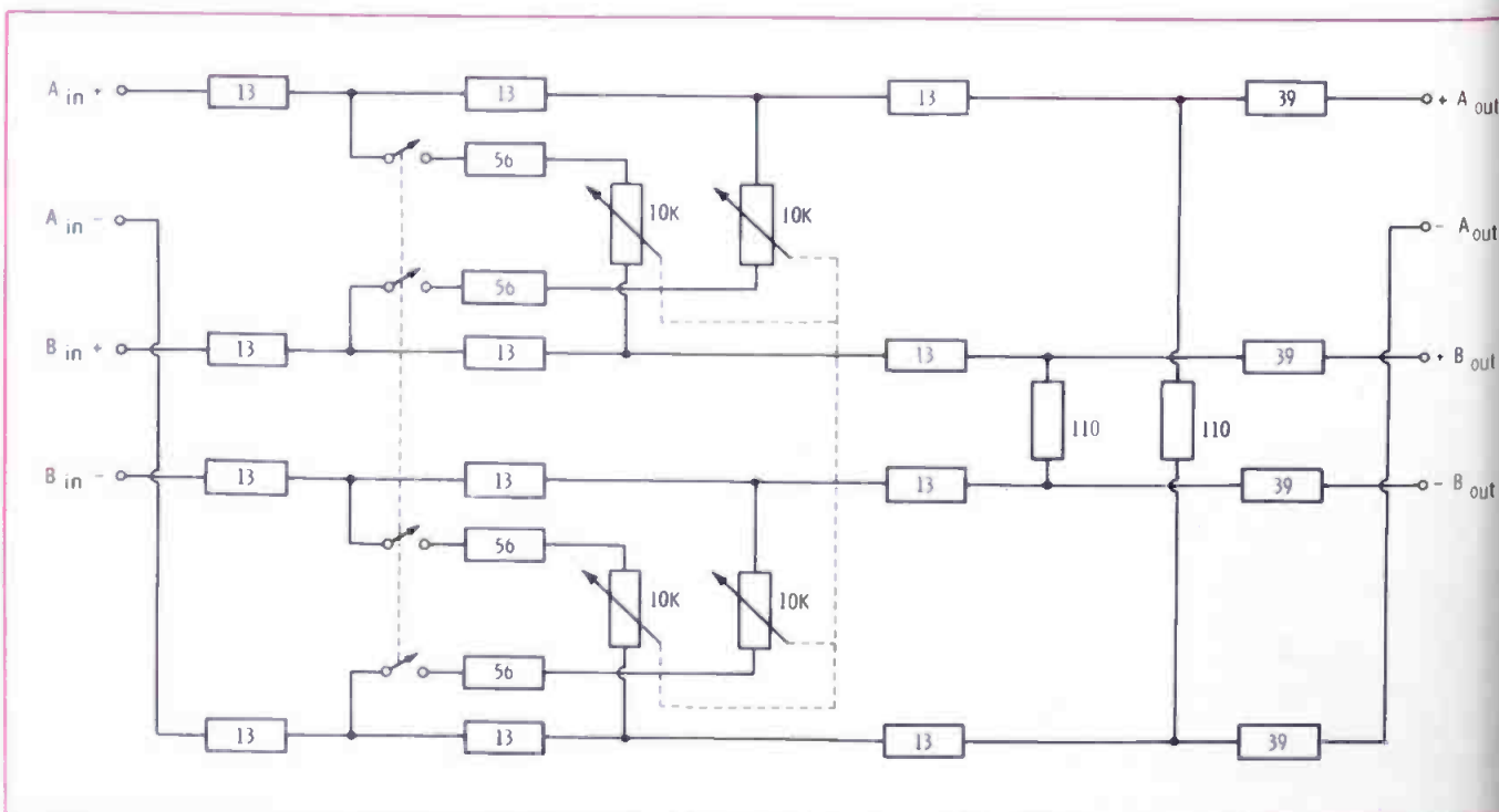
Fig. 5 Complete schematic of the circuit. If greater stereo separation is needed between channel A and B, the 10K-Ohm pot may be replaced with one of higher value. However, that would produce less control over the lower resistance range where the most audible effect takes place.
