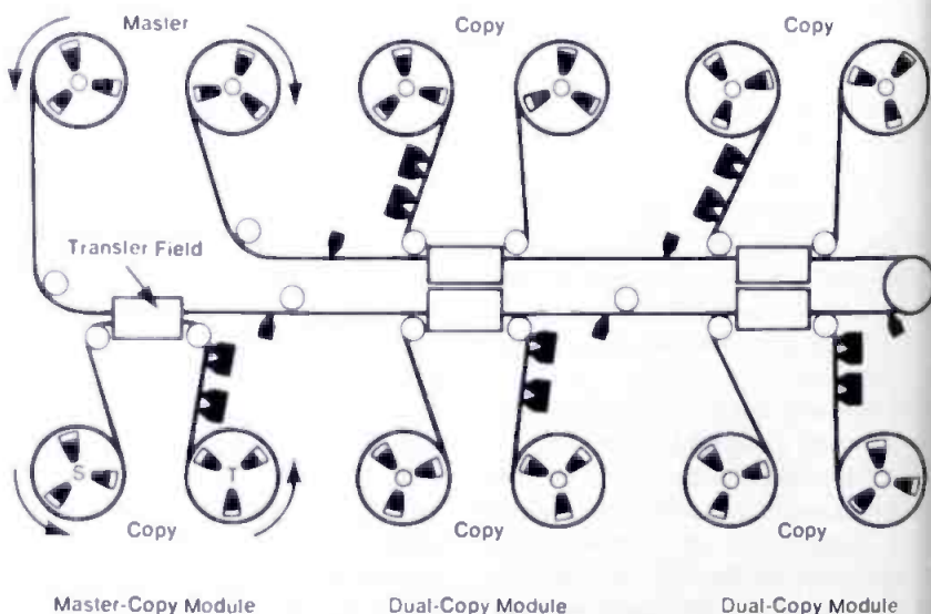
FIVE-COPY AMPEX DYNAMIC TRANSFER SYSTEM
